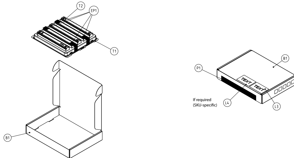
Figure 4-2: Shipping Package
